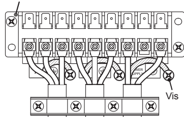
Bornier (Câble de raccordement)
