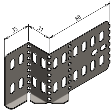
PLIAGE 30mm
