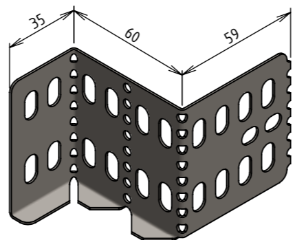
PLIAGE 60mm
