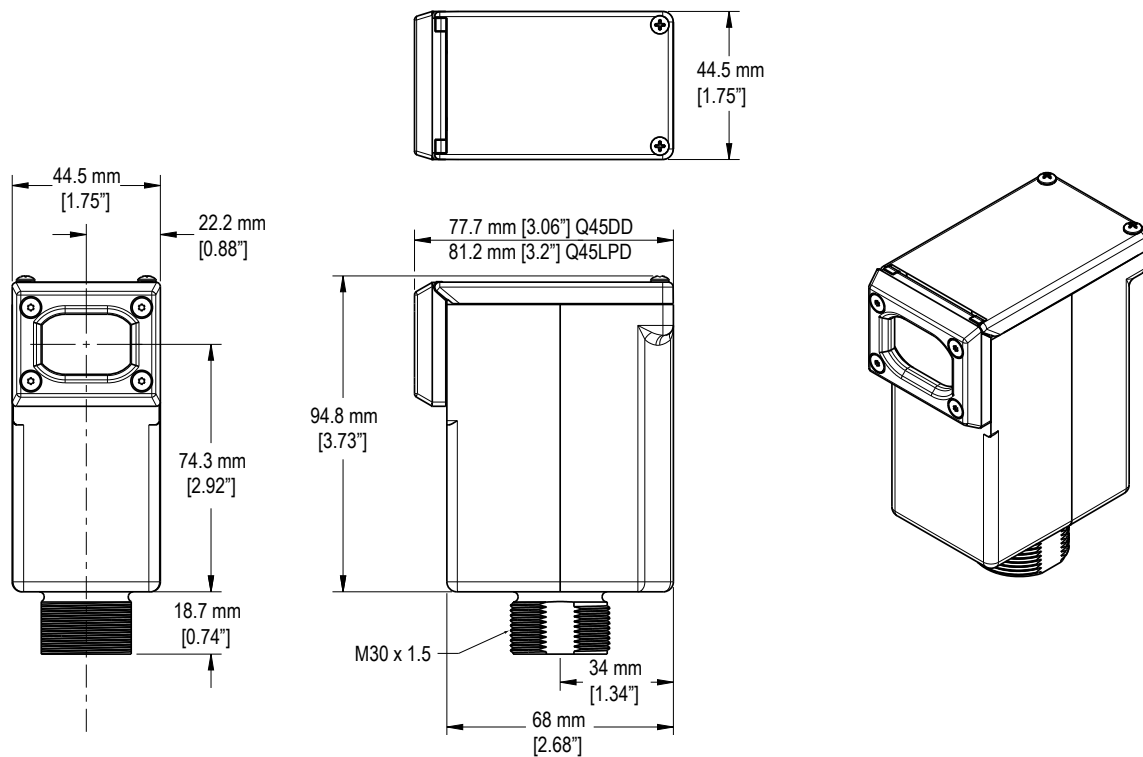
Dimensions for the Q45UPSD
