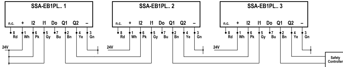
Series connection of multiple SSA-EB1PLx-0Dx.. without reset function wiring diagram.
